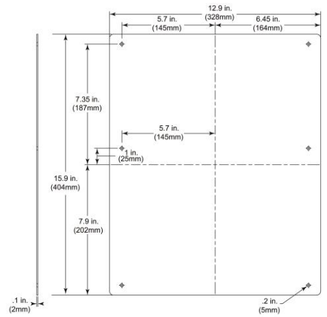
BACKPLATE STI-MBP1316
