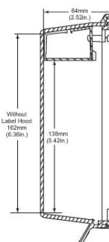
Flush Side View
