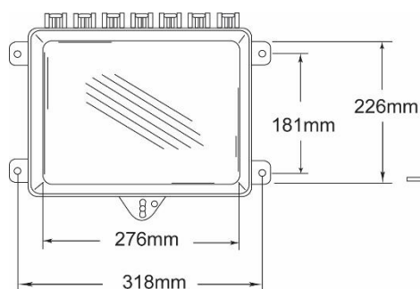
STI-7520 & STI-7521 Front View
